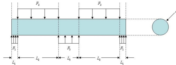
Figure 4: A beam problem in a mini-project.
