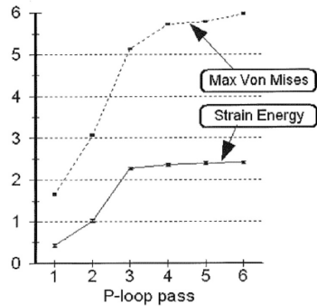
Figure 3: When the order of the p -element is increasing, the strain energy of the entire solid should be converging to a value. Otherwise, a different size of the mesh or the type of mesh should be tried for this problem.
