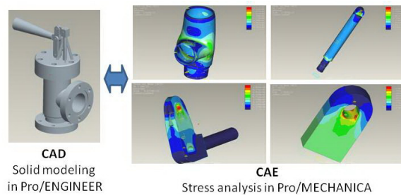
Figure 1: CAD and CAE
