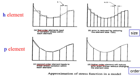
Figure 2: h -element and p -element.
