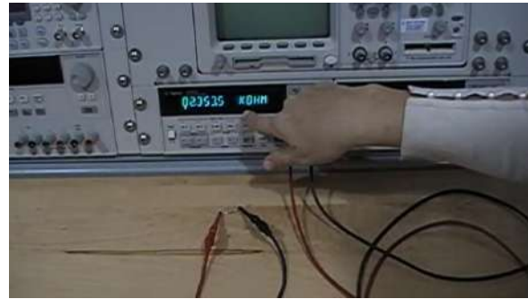
b. Instrumentation tutorial
